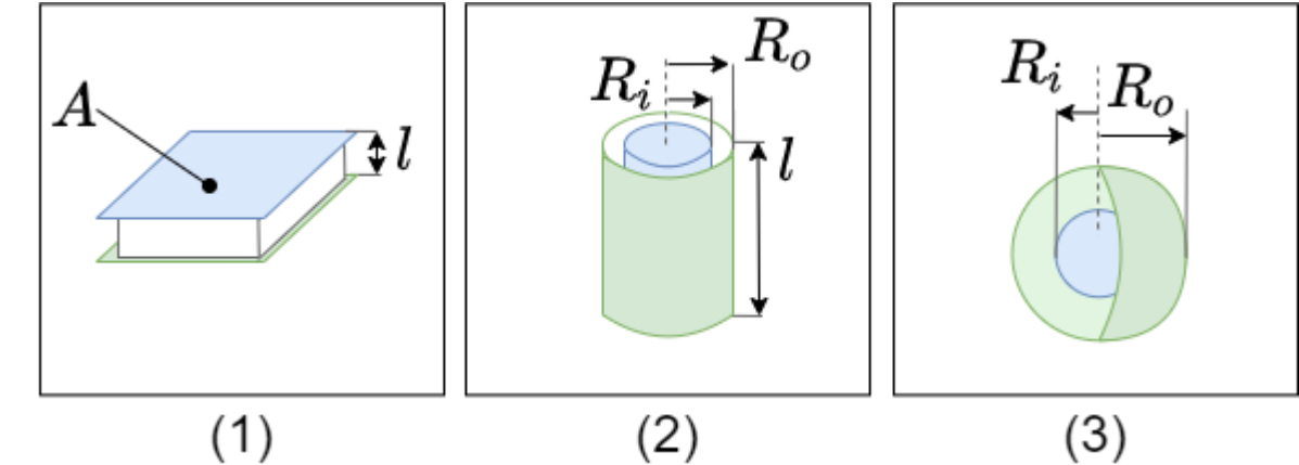
Fig. 34: geometry of capacitors
