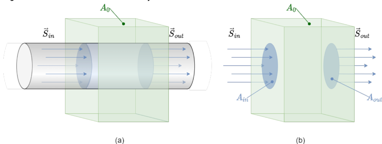
Fig. 5: Gauss's Law for Current Density
